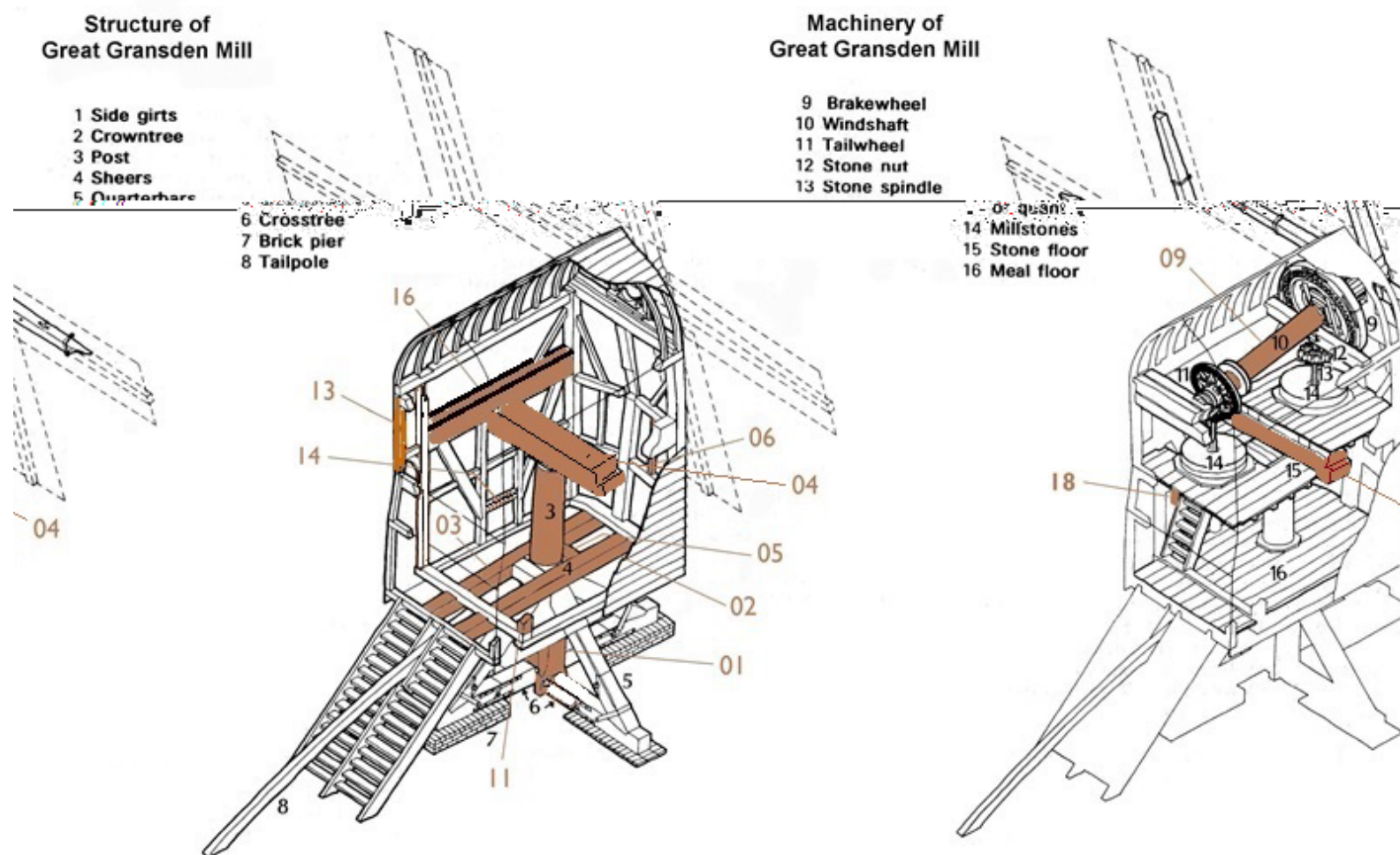
Figure 2: Timbers sampled from the mill (labelled in brown), located on isometric drawings by Graham Black
